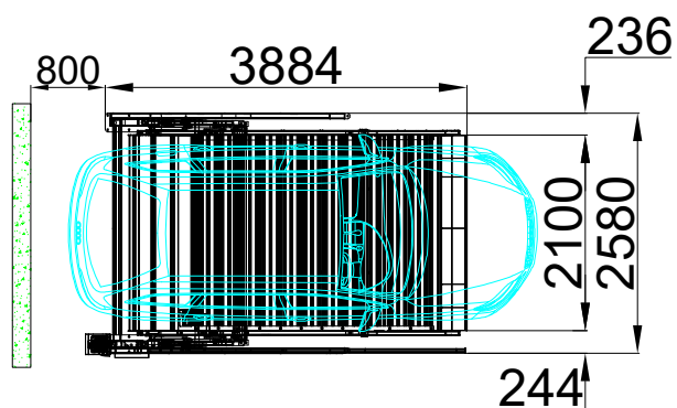
Parking plan
